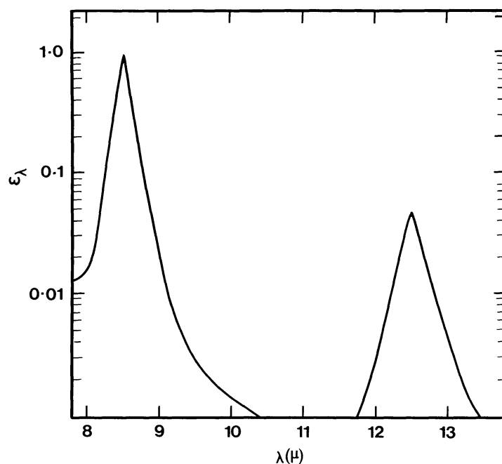
Fig. 2. Normalised absorption coefficient of silica ( \text{SiO}_2 ) spheres of radii \sim 10^{-5} cm.
