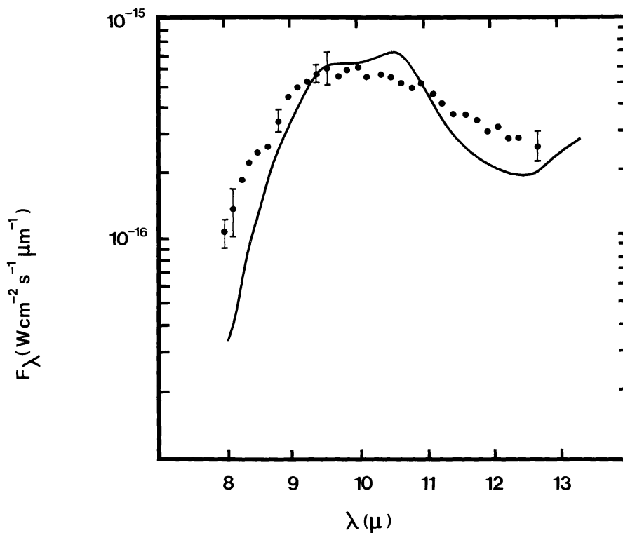
Fig. 3. Observed flux from the Trapezium Nebula (Forrest et al. , 1975a, b) compared with the behaviour of moonrock grains heated to 175 K. Moonrock data from Perry et al. (1972) for rock #14321. Normalisation is to F_{\lambda} = 6 \times 10^{-16} \text{ W cm}^{-2} \text{ s}^{-1} \mu\text{m}^{-1} at \lambda = 9.5 \mu\text{m} .
