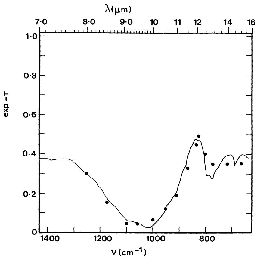
Fig. 5. Infrared transmittance of diatoms for \lambda \geq 8 \mu\text{m} compared with the best fitting values (Table I) for matching the Trapezium data.
