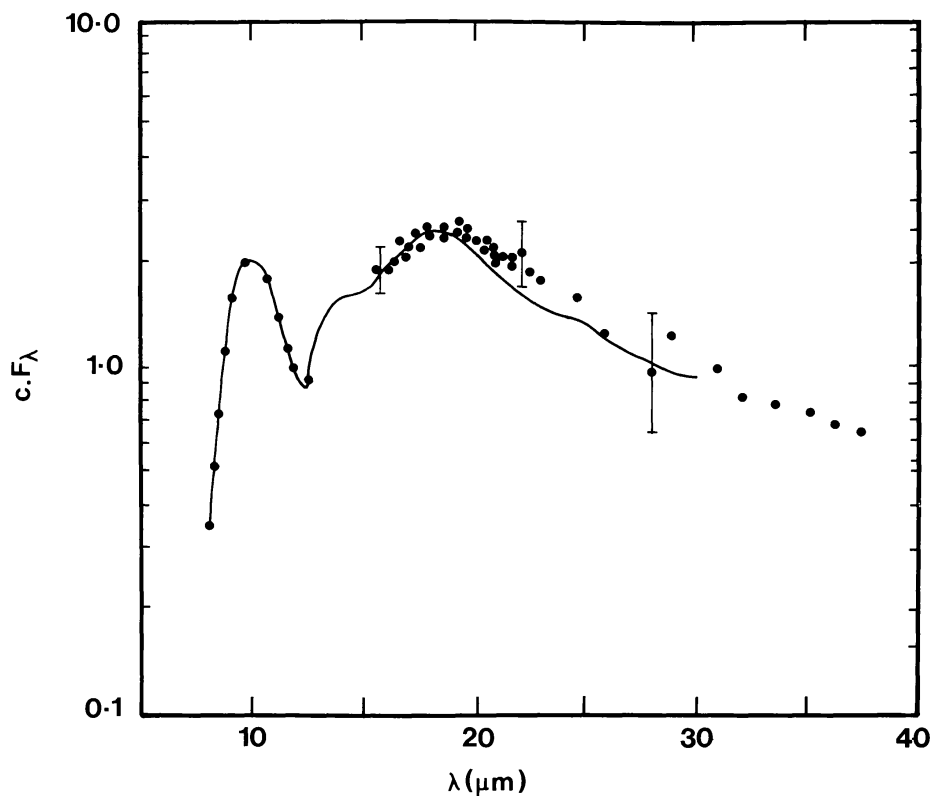
Fig. 6. The infrared spectrum of the Trapezium nebula (Forrest et al. , 1976) compared with the predicted behaviour of material resembling the diatom culture (Table I). The temperature is taken to be 175 K. Normalisation at \lambda = 9.5 \mu\text{m} .
