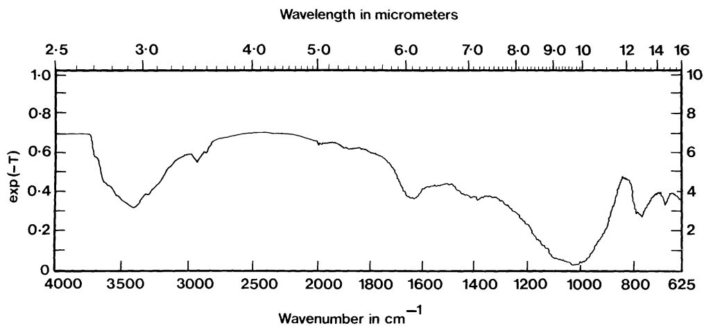
Fig. 4. Infrared spectrum of mixed diatom culture in a K Br disc.
