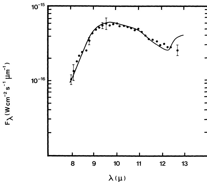
Fig. 1. Observed flux from the Trapezium Nebula (Forrest et al. , 1975a, b) compared with the behaviour of grains with opacity values set out in Table I (at a temperature of 175 K). Normalisation of curve is to F_{\lambda} = 6 \times 10^{-16} , \text{W cm}^{-2} \text{s}^{-1} \mu\text{m}^{-1} at \lambda = 9.5 \mu\text{m} .
